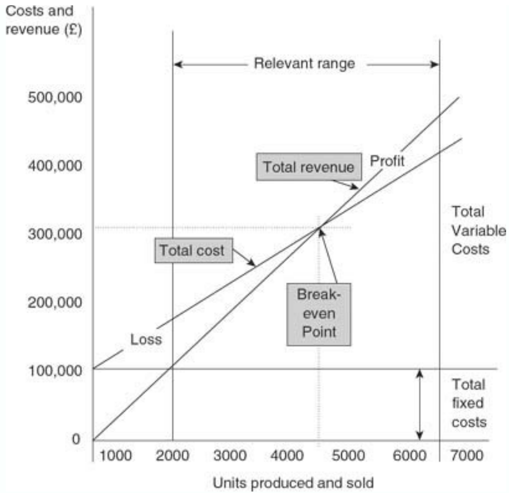
Figure 8.2 The contribution graph
