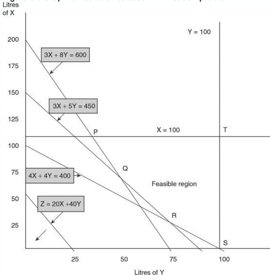
Figure 8.5 Graphical solution to cost minimisation problem
