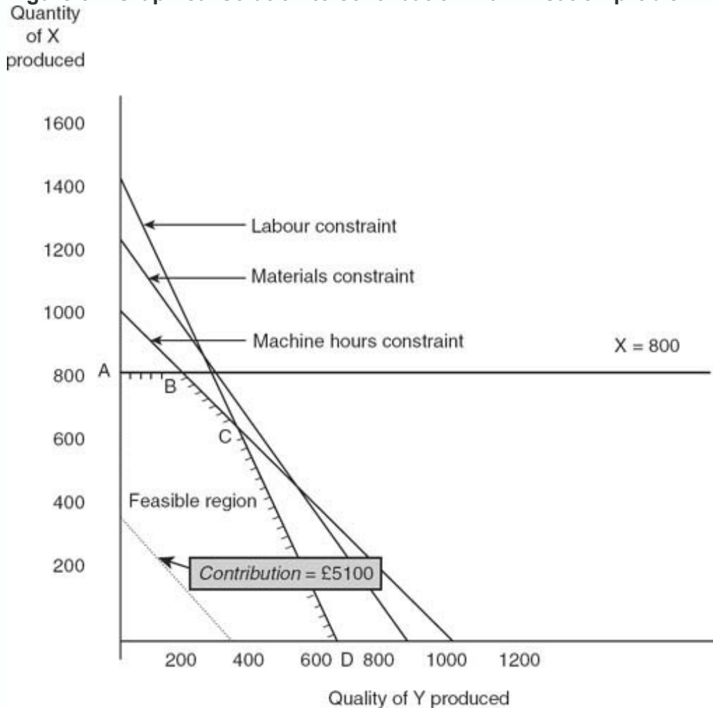
Figure 8.4 Graphical solution to contribution maximisation problem
