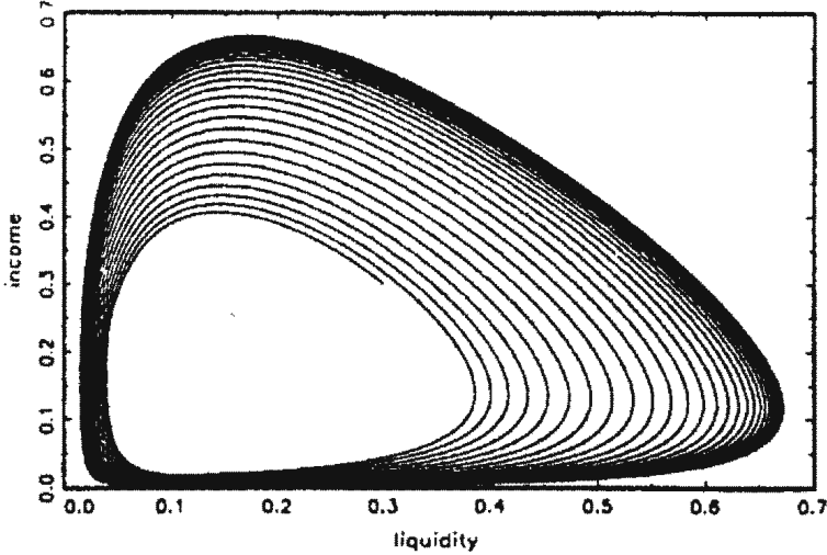
Fig. 4.1. Phase Portrait
