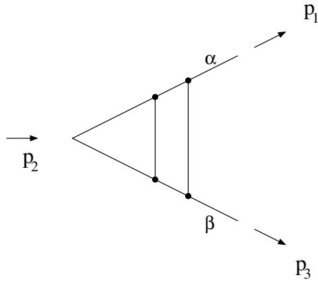
FIGURE 10. Two-loop diagram.
