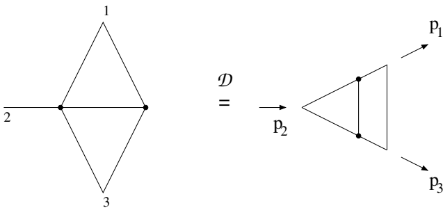
FIGURE 12. \alpha = \beta = 0 .
