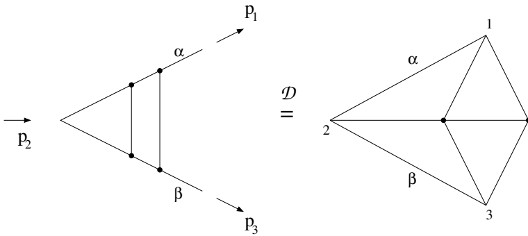
FIGURE 11. Dual representation.
