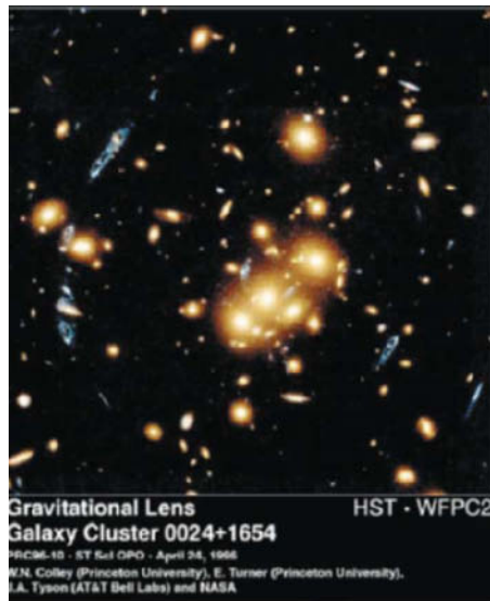
FIGURE 2. Lensing of a galaxy by a cluster of galaxies; the blue spots are all images of a single galaxy located behind the huge cluster of galaxies. (Credit: NASA, W.N. Colley (Princeton), E. Turner (Princeton) and J.A. Tyson (AT&T and Bell Labs).)
