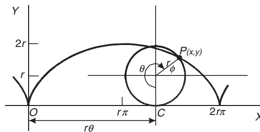
Fig. 7.3. Cycloid. The curve traced out by the point P on a circle while the circle is rolling on the x -axis
