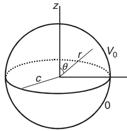
Fig. 6.9. A hollow conducting sphere
