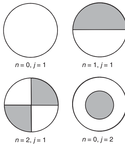
Fig. 6.4. Normal modes of drumhead vibration
