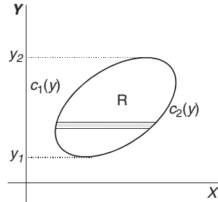
Fig. 7.11. Double integral. A double integral over the region R can be carried out by first integrating x from the left boundary x_1 = C_1(y) to the right boundary x_2 = C_2(y) with a fixed y , then integrating y from y_1 to y_2
