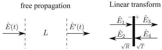
Fig. 2.2 Two basic dynamical processes of the optical field in analyzing the quantum noise of an interferometer
