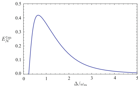
Fig. 6.4 Logarithmic negativity E_{\mathcal{N}}^{1m} as a function of the cavity modes gap \Delta \equiv \omega_1 - \omega_0 . As we can see, the condition \Delta \approx \omega_m , which optimizes the cooling, also maximizes the entanglement between the TEM 01 mode and the mechanical mode. Here we have assumed I_0 = 4.5 W (higher I_0 will make the system unstable for small \Delta ) and I_1 = 0 W. Since it can be viewed as an effective two-mode system in this case with I_1 = 0 , we simply recover the results given by Vitali et al. [19]. From Ref. [22]
