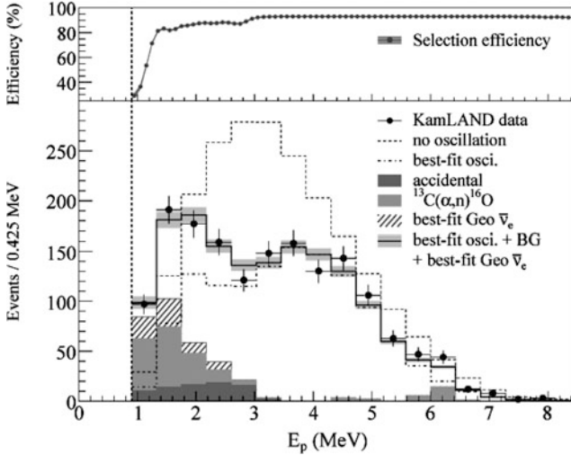
Fig. 10.4 Prompt event energy spectrum measured in the KamLAND experiment. The dashed line shows the predicted spectrum in the case of no oscillations. Best-fit oscillation curve is presented. In the shaded areas different backgrounds are shown (arXiv:0801.4589)
