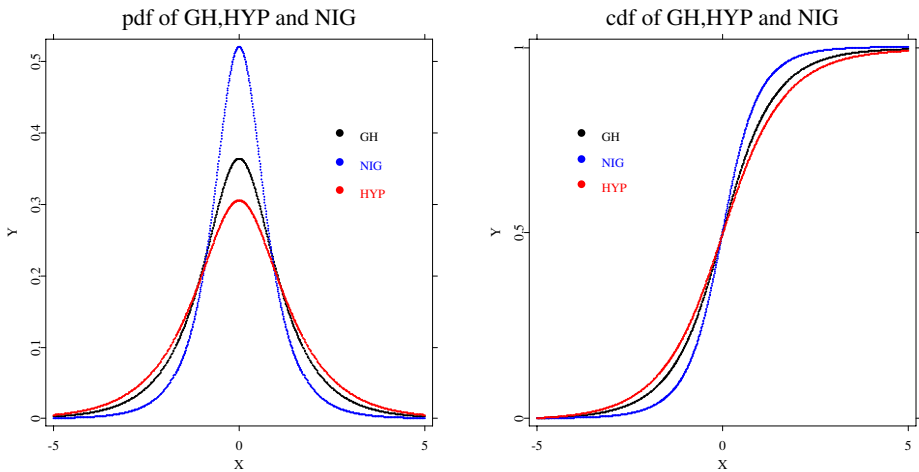
Figure 4.7. pdf (left) and cdf (right) of GH ( \lambda = 0.5 ), HYP and NIG with \alpha = 1, \beta = 0, \delta = 1, \mu = 0 MVAghdis
