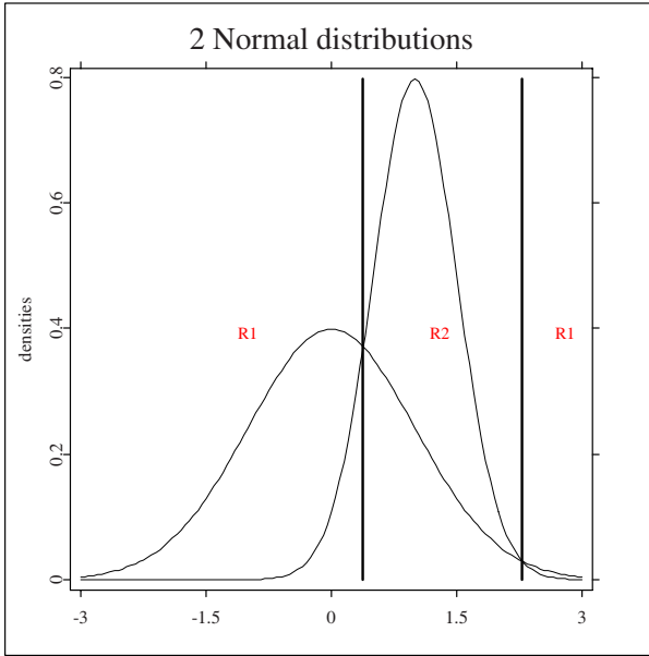
Figure 12.1. Maximum likelihood rule for normal distributions. ■ MVAdisnorm
