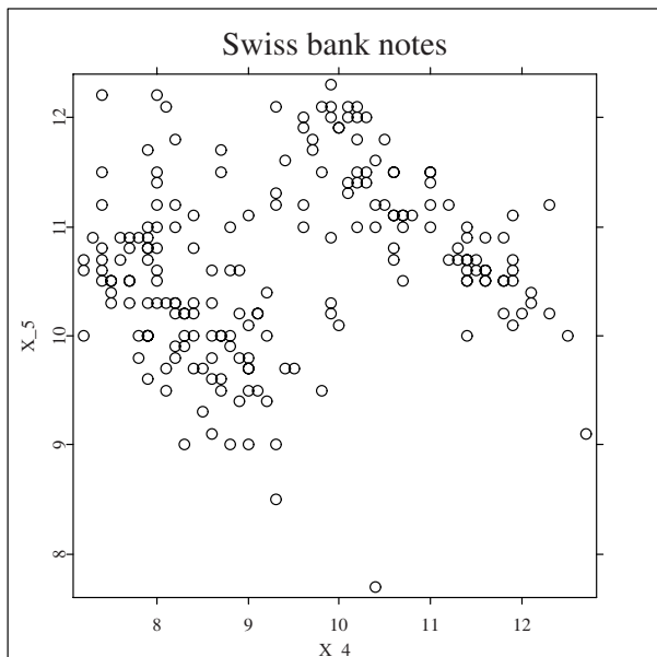
Figure 3.1. Scatterplot of variables X_4 vs. X_5 of the entire bank data set. MVA scabank45
