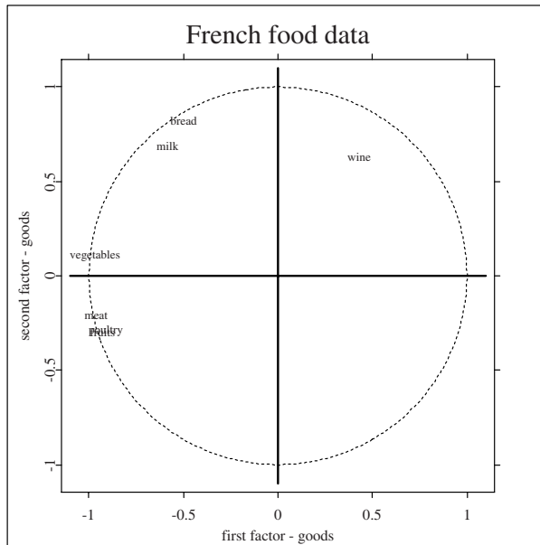
Figure 9.8. Representation of the variables. MVAnpcafood
