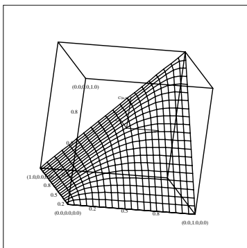
Figure 4.16. Surface plot of the Gumbel-Hougaard copula, \theta = 3 MVAghsurface
