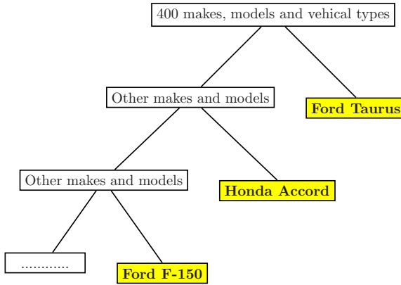
Figure 18.26. Classification tree constructed by Gini index
