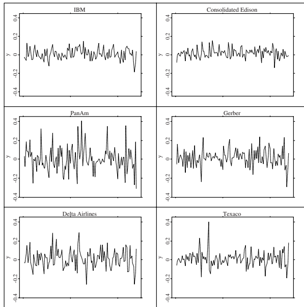
Figure 17.1. Returns of six firms from January 1978 to December 1987. ■ MVAreturns
