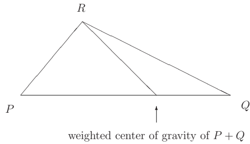
Figure 11.3. The centroid algorithm.
