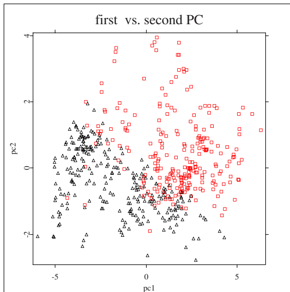
Figure 9.11. NPC analysis for the Boston housing data, scatterplot of the first two PCs. More expensive houses are marked with red color. \color{red}\square \color{black}\triangle MVAnpcahous
