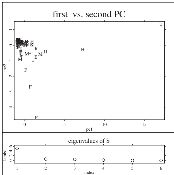
Figure 9.15. Principal components of the U.S. company data. 🔗 MVAnpcausco
