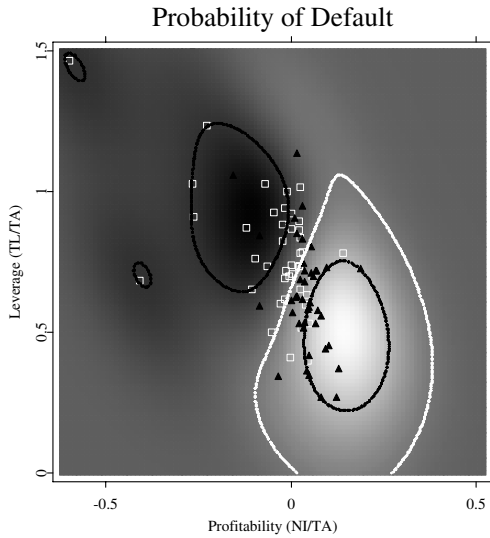
Figure 18.18. Ratings of companies in two dimensions. Optimal complexity of classifier functions (the radial basis is 1.2\Sigma^{1/2} ). The capacity is C = 1/n . Percentage of correctly cross-validated out-of-sample observations is 0.750 (maximum).
