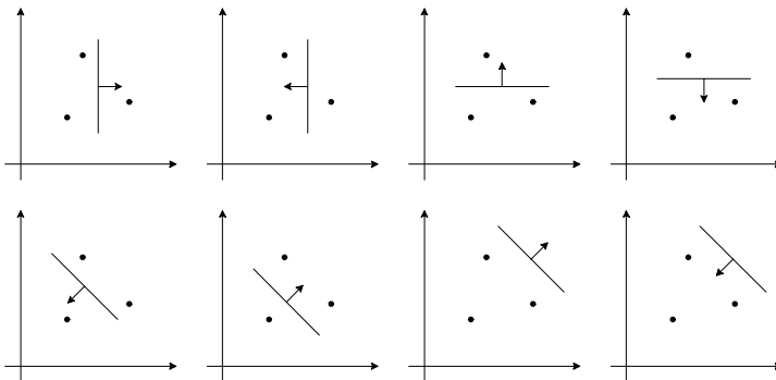
Figure 18.11. Eight possible ways of shattering 3 points on the plane with a linear indicator function.
