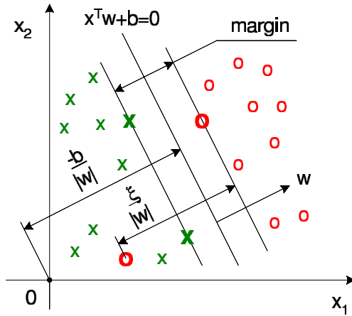
Figure 18.13. The separating hyperplane x^\top w + b = 0 and the margin in the linearly non-separable case.
