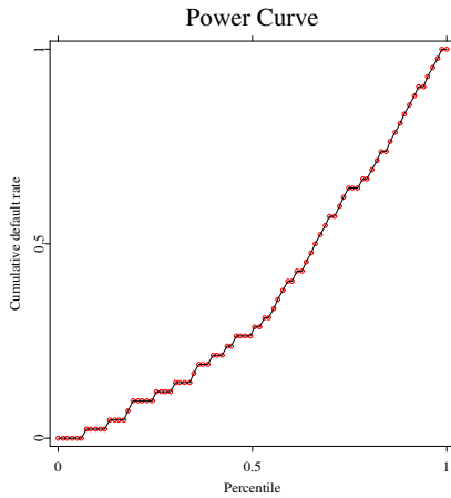
Figure 18.22. Power (Lorenz) curve (Lorenz, 1905) – the cumulative default rate as a function of the percentile of companies sorted according to their score – for the training set of companies. An SVM is applied with the radial basis 2\Sigma^{1/2} and capacity C = 1/n .
