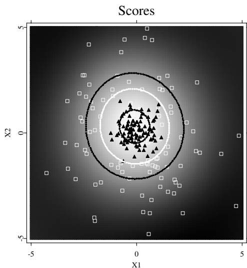
Figure 18.15. SVM classification results for the “orange peel” data ( RB = 2\Sigma^{1/2} , C = 1/n ). d = 2 , n_{-1} = n_{+1} = 100 , n = 200 ; x_{+,i} \sim N((0, 0)^\top, 2^2\mathcal{I}) , x_{-,i} \sim N((0, 0)^\top, 0.5^2\mathcal{I}) .
