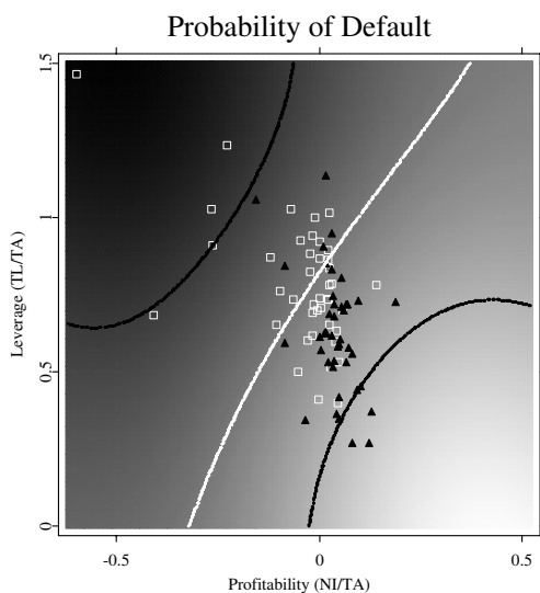
Figure 18.17. Ratings of companies in two dimensions. Low complexity of classifier functions (the radial basis is 5\Sigma^{1/2} ). The capacity is fixed at C = 1/n . Percentage of correctly cross-validated out-of-sample observations is 0.607.
