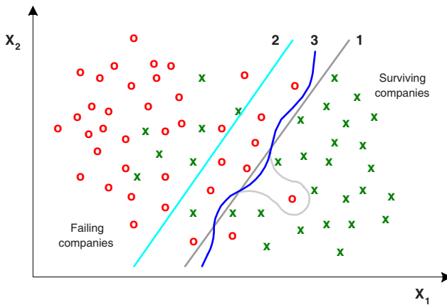
Figure 18.9. Different linear classification functions (1) and (2) and a non-linear one (3) in the linearly non-separable case.
