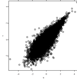
Figure 4.18. 10000-sample output for \sigma_1 = 1, \sigma_2 = 1, \theta = 3 █ MVAsample1000
