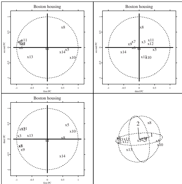
Figure 9.10. NPCA for the Boston housing data, correlations of first three PCs with the original variables. 📊 MVAnpcahausi
