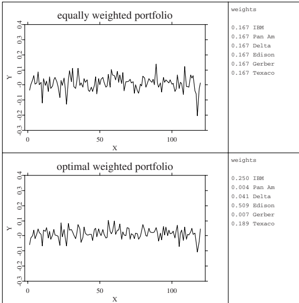
Figure 17.3. Portfolio of all six assets, equal and efficient weights. MVAportfol
