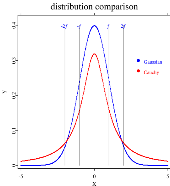
Figure 4.6. Comparison of the pdf of a standard Gaussian (blue) and a Cauchy distribution (red) with location parameter 0 and scale parameter 1. MVGausscauchy
