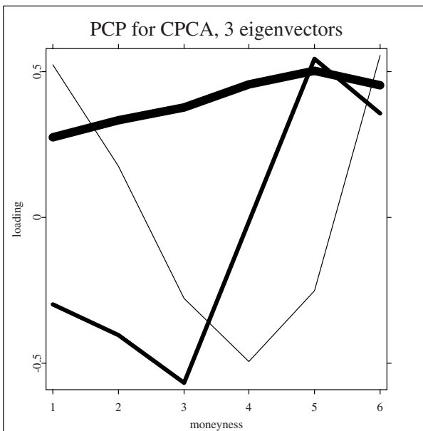
Figure 9.9. Factor loadings of the first (thick), the second (medium), and the third (thin) PC \blacksquare MVAcpcaiv
