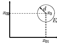
Figure 2.2. Iso-distance sphere.
