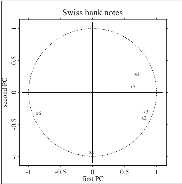
Figure 9.14. The correlations of the original variable with the PCs. MVAnpcabanki
