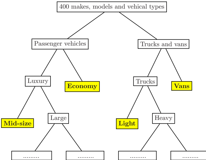
Figure 18.27. Classification tree constructed by twoling index
