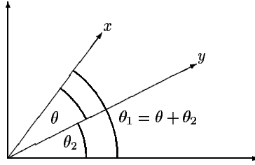
Figure 2.4. Angle between vectors.
