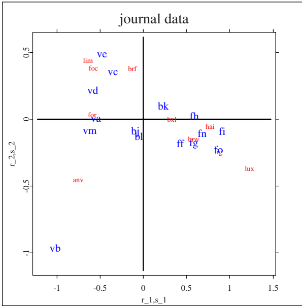
Figure 13.1. Projection of rows (the 15 newspapers) and columns (the 10 regions) \blacksquare MVAcorrjour
