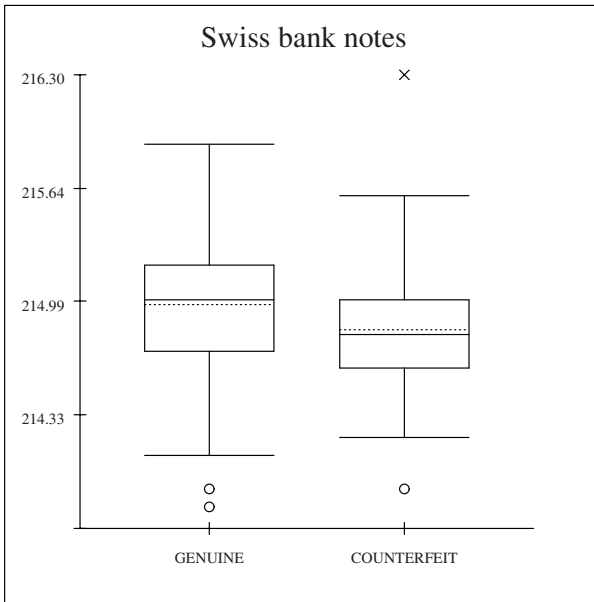
Figure 1.5. The X_1 variable of Swiss bank data (length of bank notes).
