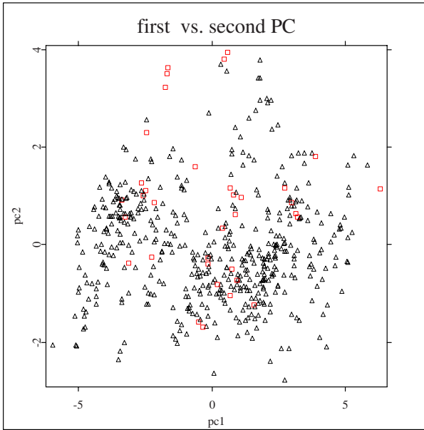
Figure 9.12. NPC analysis for the Boston housing data, scatterplot of the first two PCs. Houses close to the Charles River are indicated with red squares. \blacksquare MVA npca housing
