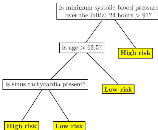
Figure 18.23. Decision tree for low/high patients
