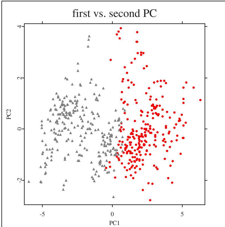
Figure 11.10. Scatterplot of the first two PCs displaying the two clusters.
