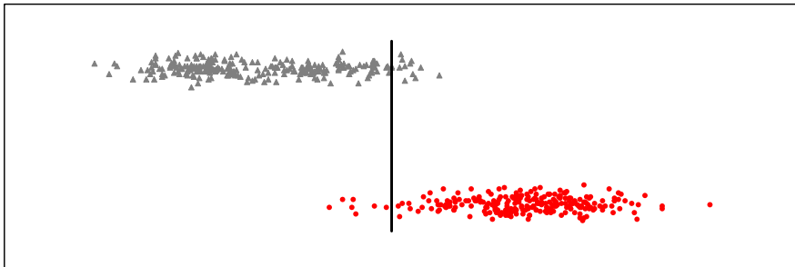
Figure 12.3. Discrimination scores for the two clusters created from the Boston housing data. MVAdiscbh
