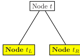
Figure 18.25. Parent and child nodes hierarchy
