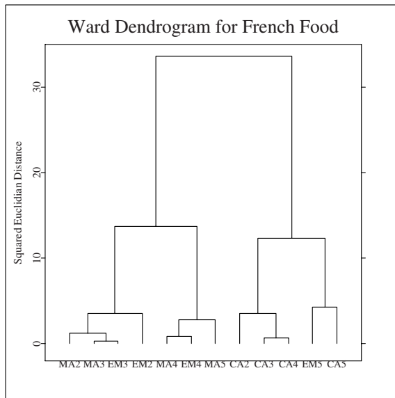
Figure 11.6. The dendrogram for the French food expenditures, Ward algorithm. MVAclusfood
