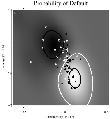
Figure 18.20. Ratings of companies in two dimensions. Low capacity ( C = 0.3/n ). The radial basis is fixed at 1.2\Sigma^{1/2} . Percentage of correctly cross-validated out-of-sample observations is 0.714.
