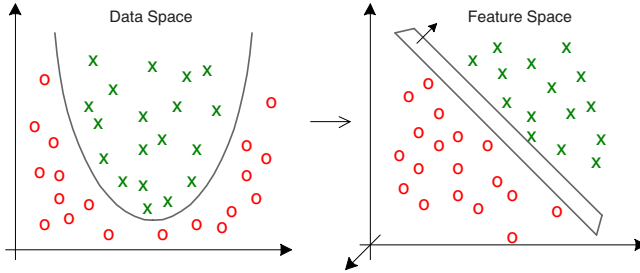
Figure 18.14. Mapping into a three dimensional feature space from a two dimensional data space \mathbb{R}^2 \mapsto \mathbb{R}^3 . The transformation \Psi(x_1, x_2) = (x_1^2, \sqrt{2}x_1x_2, x_2^2)^\top corresponds to the kernel function K(x_i, x_j) = (x_i^\top x_j)^2
