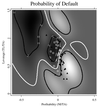
Figure 18.21. Ratings of companies in two dimensions. High capacity ( C = 10/n ). The radial basis is fixed at 1.2\Sigma^{1/2} . Percentage of correctly cross-validated out-of-sample observations is 0.631.
