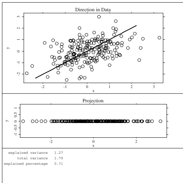
Figure 9.2. The most interesting SLC. MVApCasimu
