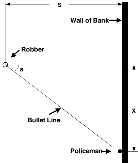
Figure 4.10. Introduction to Cauchy distribution - robber vs. policeman
