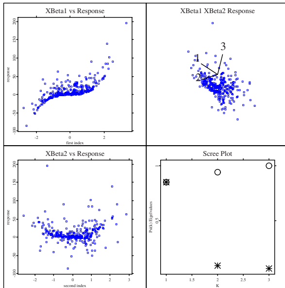
Figure 18.4. SIR: The left plots show the response versus the estimated EDR-directions. The upper right plot is a three-dimensional plot of the first two directions and the response. The lower right plot shows the eigenvalues \hat{\lambda}_i (*) and the cumulative sum (o). ■ MVA sir data
