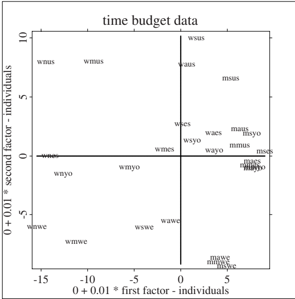
Figure 9.18. Representation of the individuals. ■ MVAnpcatime
