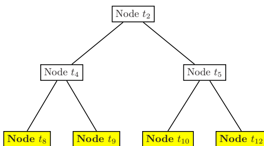
Figure 18.28. Decision tree hierarchy
