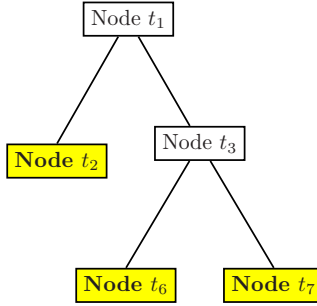
Figure 18.30. T - T_{t_2} the pruned tree T
