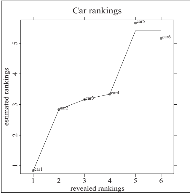
Figure 16.1. Plot of estimated preference orderings vs. revealed rankings and PAV fit. ■ MVAcarrankings
