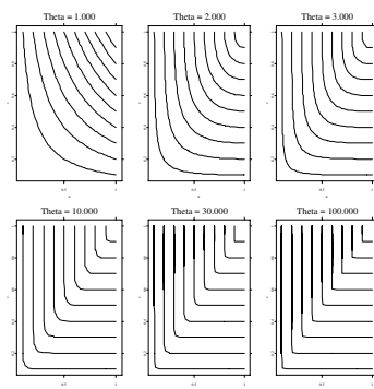
Figure 4.17. Contour plots of the Gumbel-Hougaard copula MVAghtour
