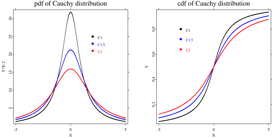
Figure 4.11. pdf (left) and cdf (right) of Cauchy distribution with m = 0 and different scale parameters (C1 stands for Cauchy distribution with s = 1 ) MVAcauchy
