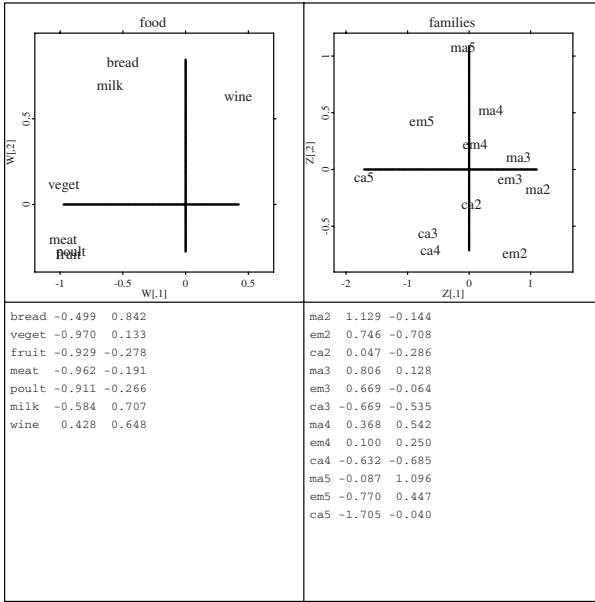
Figure 8.6. Representation of food expenditures and family types in two dimensions. MVAdecofood
