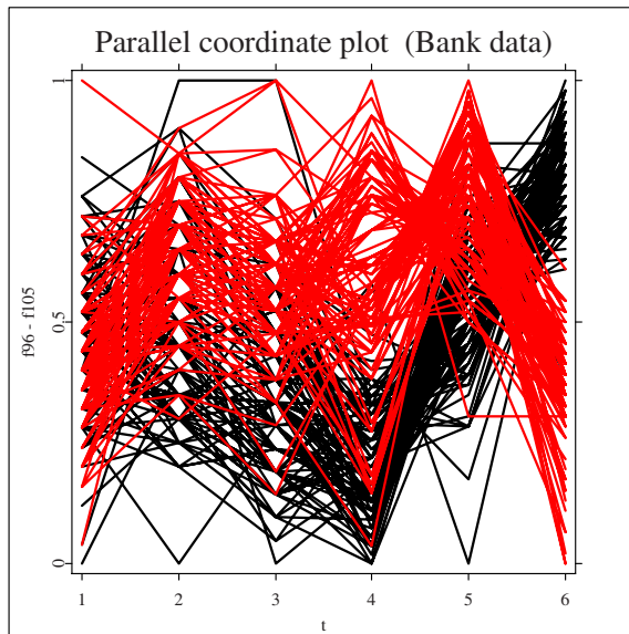
Figure 1.23. The entire bank data set. Genuine bank notes are displayed as black lines. The counterfeit bank notes are shown as red (grey) lines.
