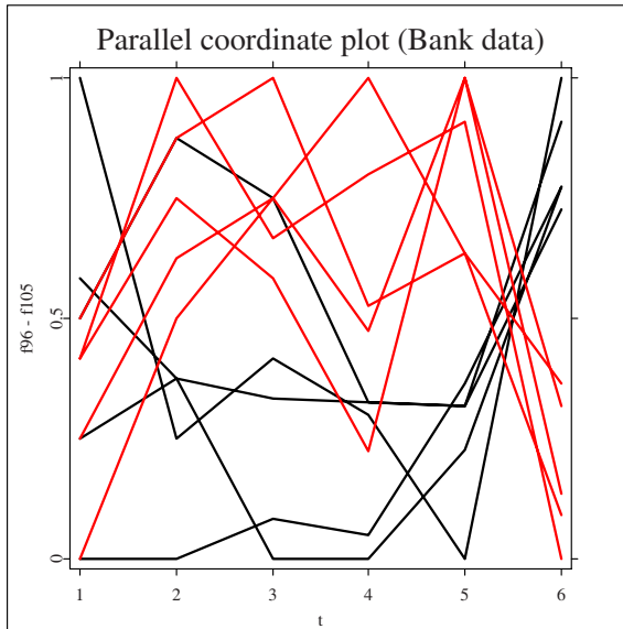
Figure 1.22. Parallel coordinates plot of observations 96–105. MVAparcoo1
