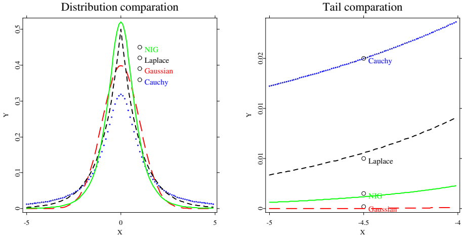
Figure 4.15. Graphical comparison of the NIG distribution (line), standard normal distribution \bullet MVAgdata tail
