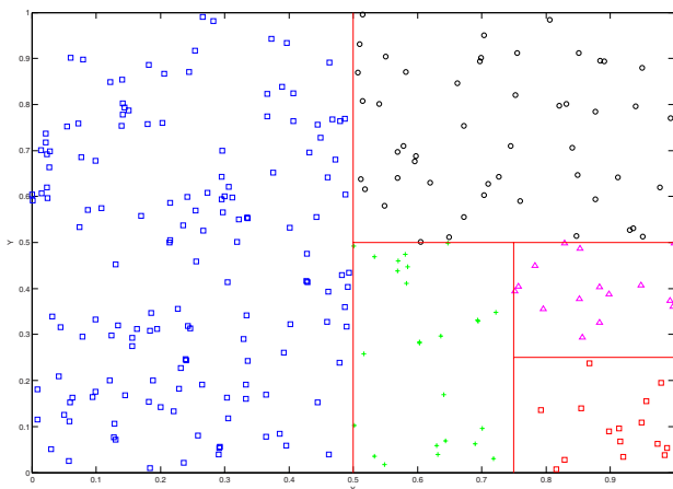
Figure 18.24. CART orthogonal splitting example where each color corresponds to one cluster
