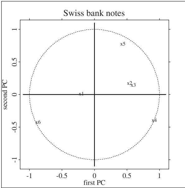
Figure 9.6. The correlation of the original variable with the PCs. MVApcabanki
