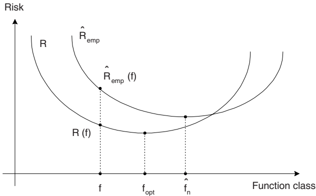
Figure 18.10. The minima f_{opt} and \hat{f}_n of the expected ( R ) and empirical ( \hat{R} ) risk functions generally do not coincide.
