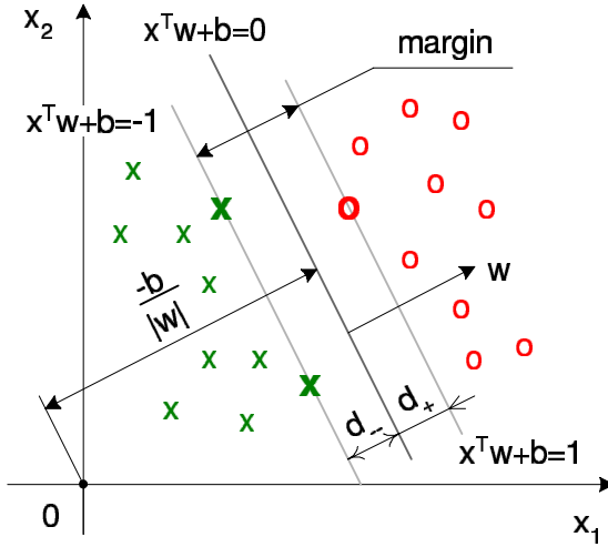
Figure 18.12. The separating hyperplane x^T w + b = 0 and the margin in the linearly separable case.
