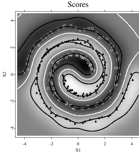
Figure 18.16. SVM classification results for the noisy spiral data ( RB = 0.4\Sigma^{1/2} , C = 1.2/n ). The spirals spread over 3\pi radian; the distance between the spirals equals 1.0. d = 2 , n_{-1} = n_{+1} = 100 , n = 200 . The noise was injected with the parameters \varepsilon_i \sim N(0, 0.1^2\mathcal{I}) . The separation is perfect.
