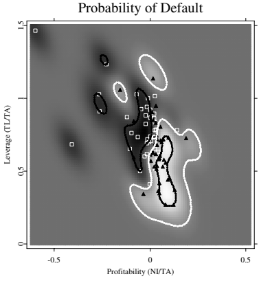
Figure 18.19. Ratings of companies in two dimensions. Excessively complex classification functions (the radial basis is 0.5\Sigma^{1/2} ). The capacity is fixed at C = 1/n . Percentage of correctly cross-validated out-of-sample observations is 0.690.
