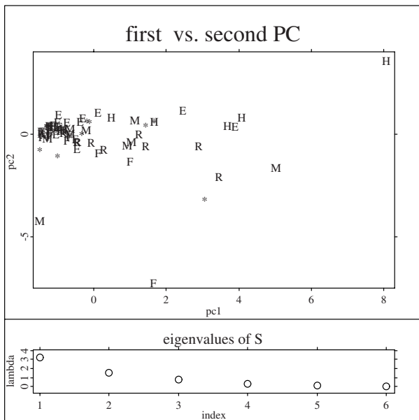
Figure 9.16. Principal components of the U.S. company data (without IBM and General Electric). \bullet MVAnpcausco2
