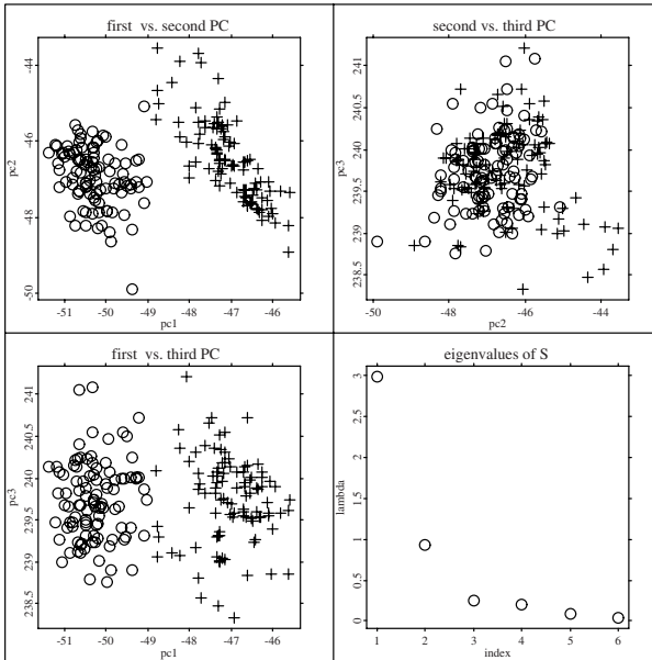
Figure 9.3. Principal components of the bank data. \circ MVApccabank
