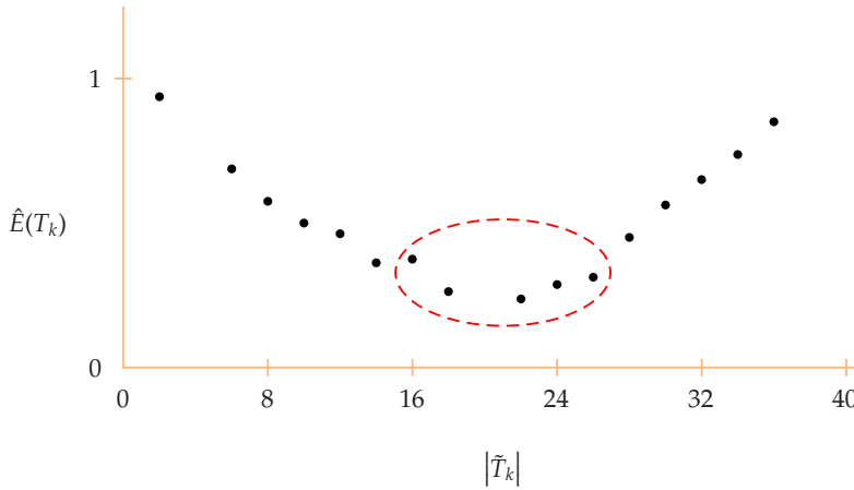
Figure 18.31. The example of relationship between \hat{E}(T_k) and number of terminal nodes
