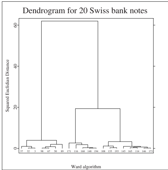
Figure 11.5. The dendrogram for the 20 bank notes, Ward algorithm. MVAclusbank
