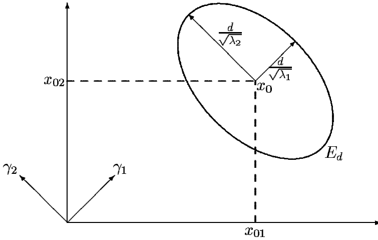
Figure 2.3. Iso-distance ellipsoid.
