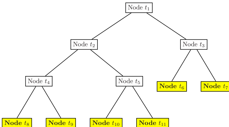
Figure 18.28. Decision tree hierarchy
