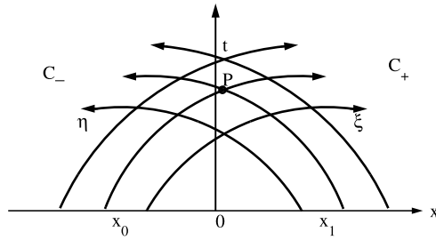
Fig. 6.21 Characteristics C_{\pm} .
