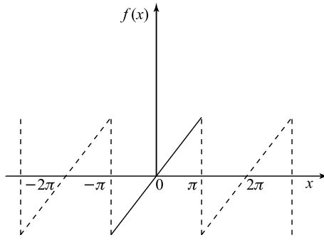
Fig. B.4 The sawtooth wave function.
