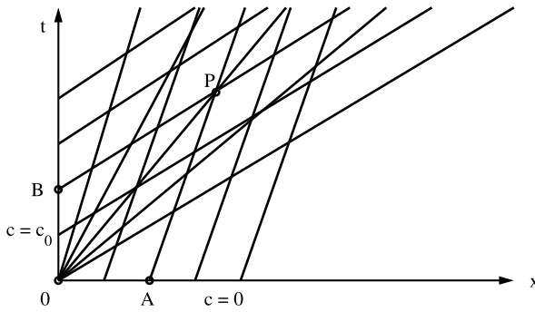
Fig. 6.11 Overlapping characteristic lines.
