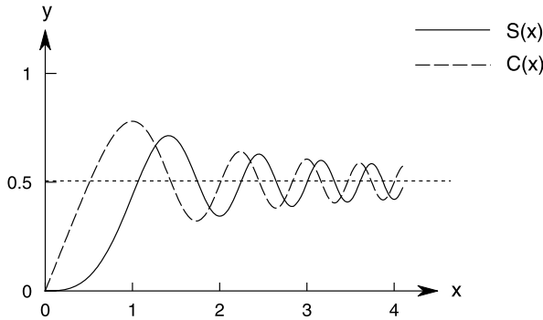
Fig. A.3 The Fresnel integrals C(x) and S(x) .
