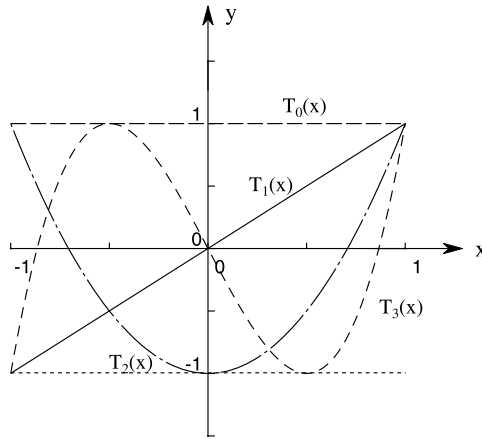
Fig. A.9 Chebyshev polynomials y = T_n(x) .
