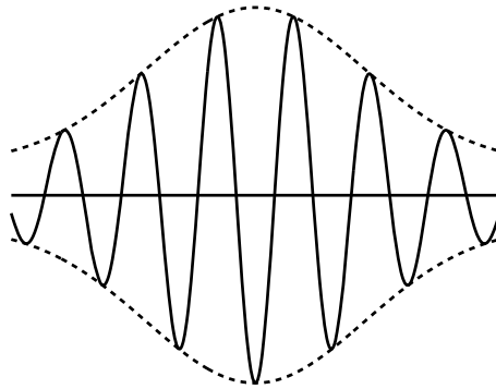
Fig. 10.1 An envelope soliton.
