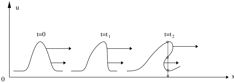
Fig. 5.4 Distortion of wave profile with increasing time t_2 \gg t_1 > 0 .
