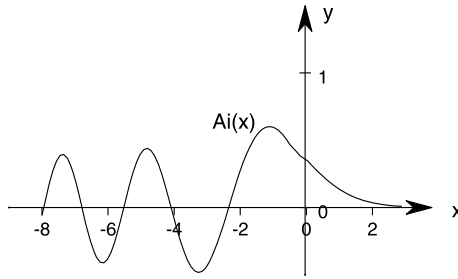
Fig. A.7 The Airy function.
