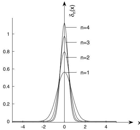
Fig. B.8 The sequence of delta functions, \delta_n(x) .
