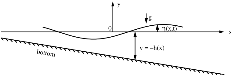
Fig. 6.20 Long surface waves in shallow water.
