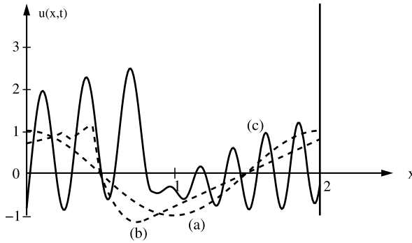
Fig. 9.2 Development of solitary waves: (a) initial profile at t = 0 , (b) profile at t = \pi^{-1} , and (c) wave profile at t = (3.6)\pi^{-1} . From Zabusky and Kruskal (1965).
