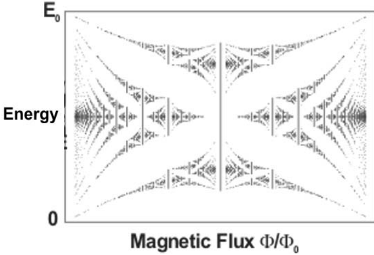
FIGURE 9. Hofstadter butterfly
