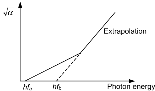
Fig. 10.4. Indirect transitions: hf_a = E_g - E_{\text{phonon}} , hf_b = E_g + E_{\text{phonon}} , E_g = (hf_a + hf_b)/2 , sketch
