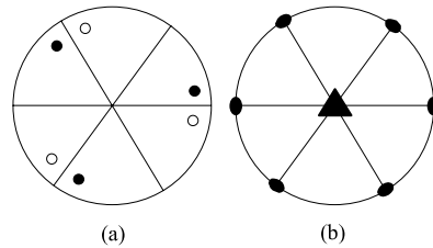
Fig. 1.18. Illustration of the way a stereogram is constructed
