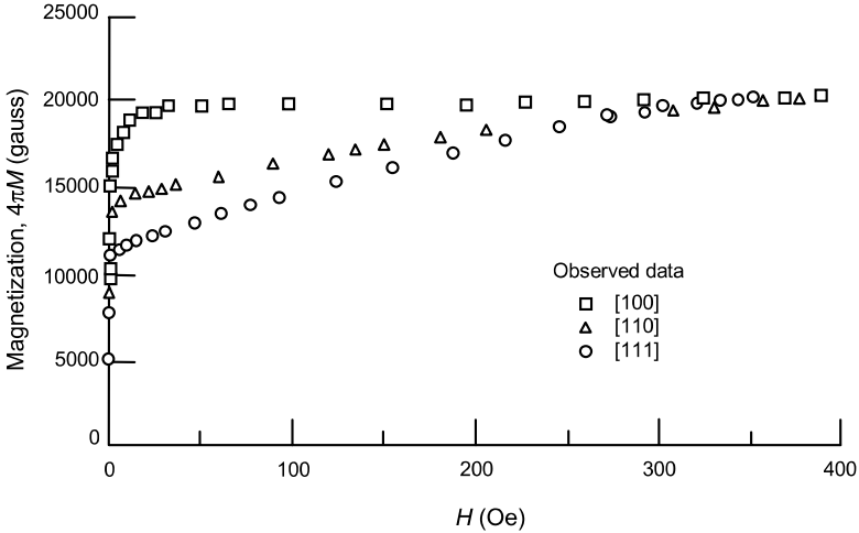
Fig. 7.19. Magnetization curves showing anisotropy for single crystals of iron with 3.85% silicon [Reprinted with permission from Williams HJ, Phys Rev 52 (7), 747 (1937). Copyright 1937 by the American Physical Society.]
