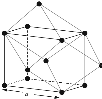
b) Conventional and primitive cells of bcc lattice
