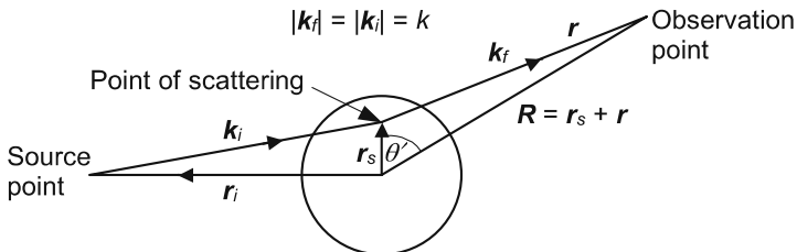
Fig. 1.25. Plane-wave scattering
