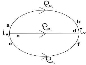
FIGURE 4. A spin network
