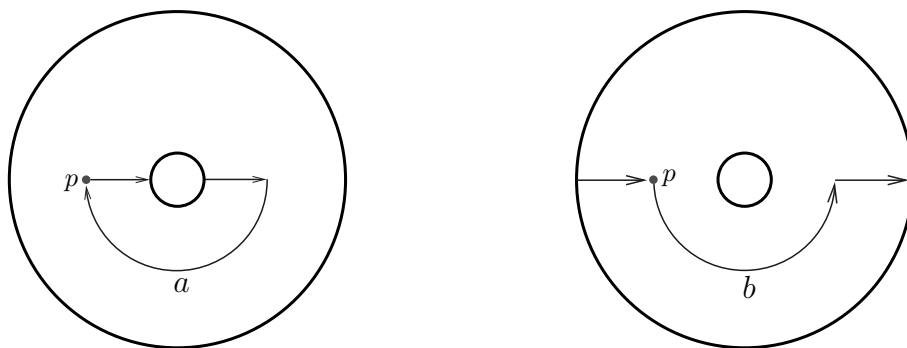
FIGURE 7. Loops a (left picture) and b (right picture) in \mathbb{R}P^3 \natural \mathbb{R}P^3 that generate the fundamental group \mathbb{Z}_2 * \mathbb{Z}_2 = \langle a, b : a^2 = b^2 = 1 \rangle based at point p . The product loop, c := ab (first a then b ), is homotopic to the loop \ell in Fig. 6, that is, to a circle fiber.
