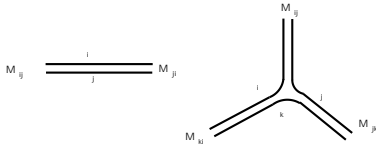
FIGURE 1. Propagator and vertex
