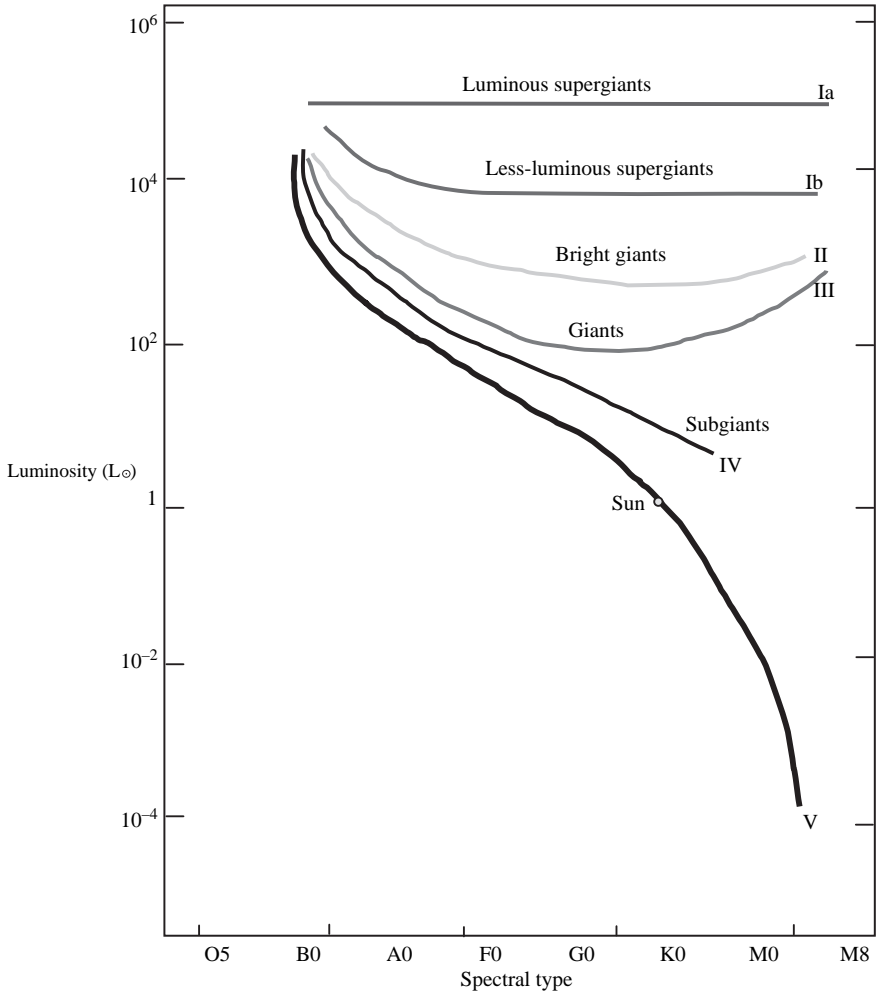
Figure 1.6. Luminosity classes. Dividing the H - R diagram according to luminosity classes allows distinctions to be made between giant and supergiant stars.
