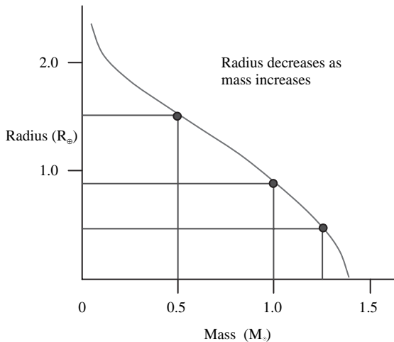
Figure 3.24. Mass-radius relationship for white dwarf stars.
