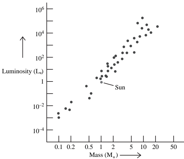
Figure 3.4. Mass-luminosity relationship.
