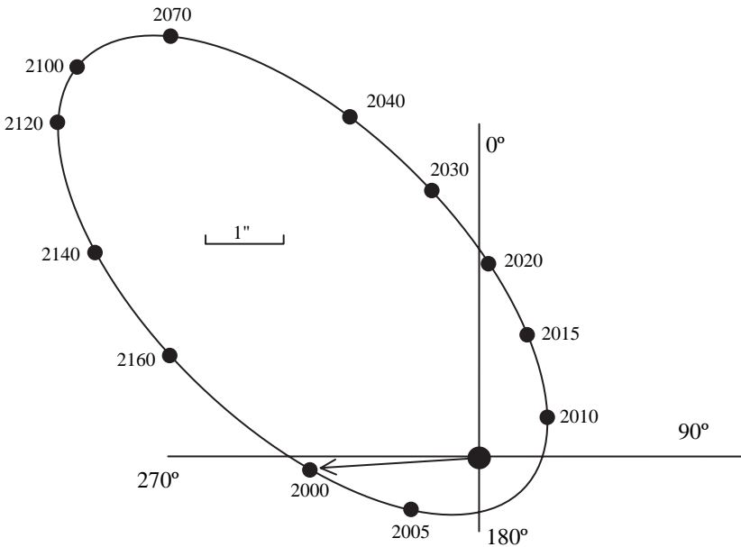
Figure 3.9. Separation and position angle of \gamma Virginis.
