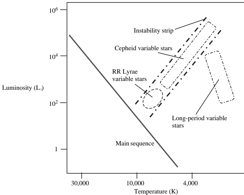
Figure 3.17. Variable stars on the H - R diagram.
