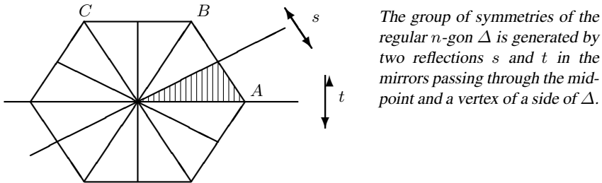
Fig. 7.1. For the proof of Theorem 7.2.
