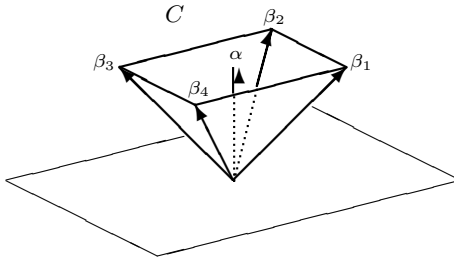
Fig. 4.2. Extreme and nonextreme vectors
