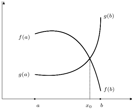
Fig. 20.3. The intermediate value theorem: if f and g are continuous functions on [a, b] and f(a) > g(a) , f(b) < g(b) , then there exists a point x_0 \in [a, b] such that f(x_0) = g(x_0) .
