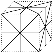
\{1\} -residues cosets of \langle r_1 \rangle
