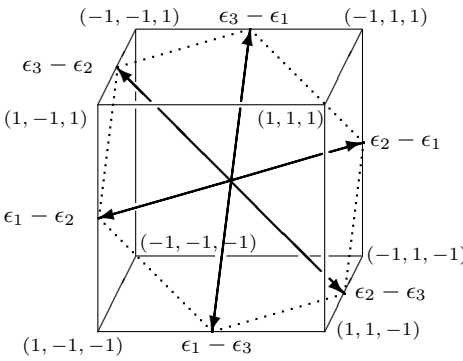
Fig. 9.2. Root system of type A_2
