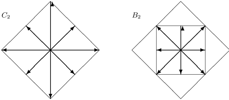
Fig. 9.5. Root systems B_2 and C_2 .
