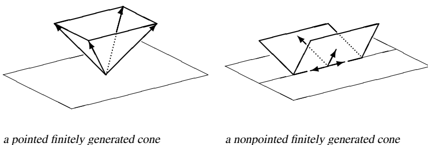
Fig. 4.1. Pointed and nonpointed cones.
