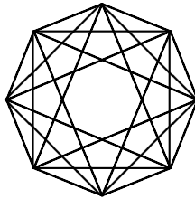
Fig. 9.8. 2-dimensional projection of a 4-dimensional cross polytope.
