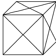
\{3\} -residues cosets of \langle r_3 \rangle
