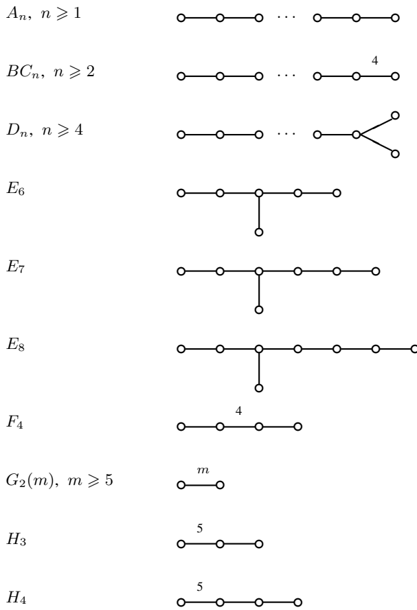
Fig. 16.1. Positive definite graphs.
