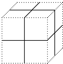
\{1, 2\} -residues cosets of \langle r_1, r_2 \rangle
