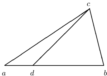
Fig. 2.1. For the proof of Theorem 2.1.
