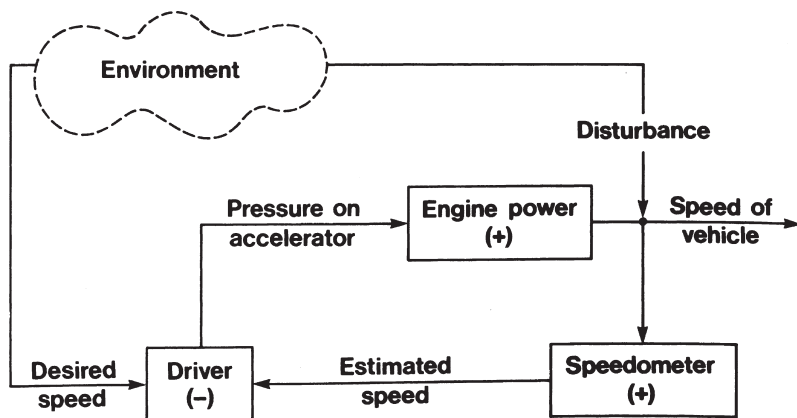
Fig. 1.7 Feedback control of an automobile
