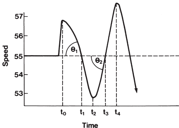
Fig. 1.11 The results of overcompensation for a disturbance in the speed of a vehicle
