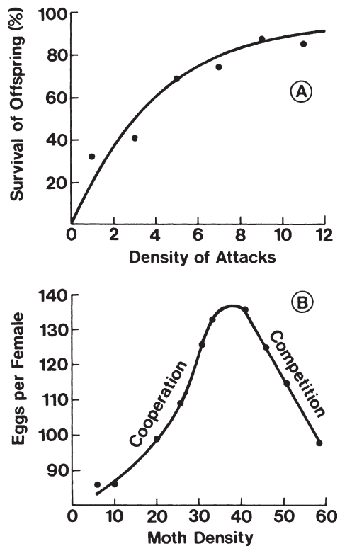
Fig. 3.3 (A) Effect of bark beetle attack density on the survival of its offspring from the defense secretions of its coniferous host (redrawn after A. A. Berryman. Environmental Entomology , vol. 3, p. 579. 1974). (B) Effect of population density on the number of eggs laid by flour moth females (redrawn from G. C. Ulyett, Journal of the Entomological Society of South Africa , vol. 8, p. 53, 1945)
