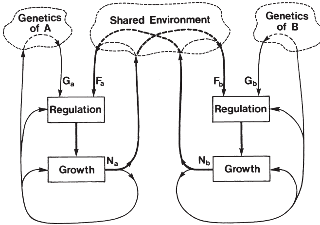
Fig. 4.1 A general model for two interacting species, A and B, where the numbers of the first species, N_a , affect the favorability of the other species' environment, F_b , and vice versa; the G 's indicate genetic properties of the two species
