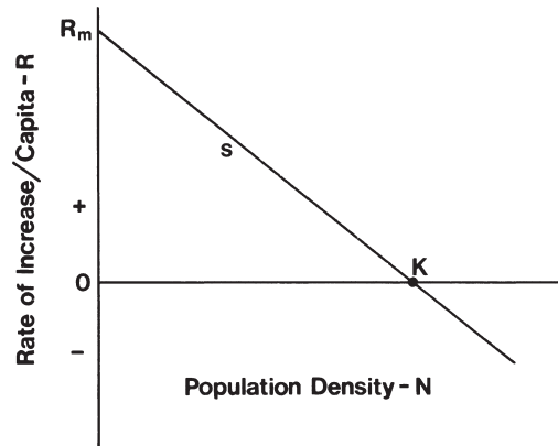
Fig. 2.12 A linear relationship between the individual rate of increase, R , and population density, N , where R_m is the maximum per capita rate of increase, s is the slope of the relationship, and K is the equilibrium density
