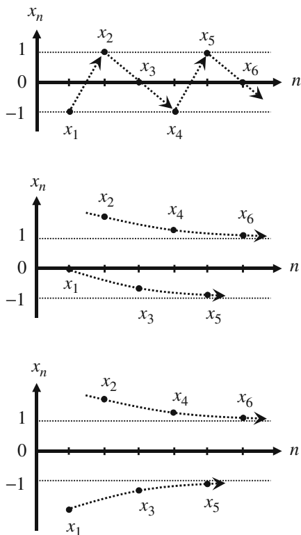
Fig. 2.1. All the sequences of \{x_n\} in the figures do not converge, but they all possess \limsup_{n \rightarrow \infty} x_n = 1 and \liminf_{n \rightarrow \infty} x_n = -1
