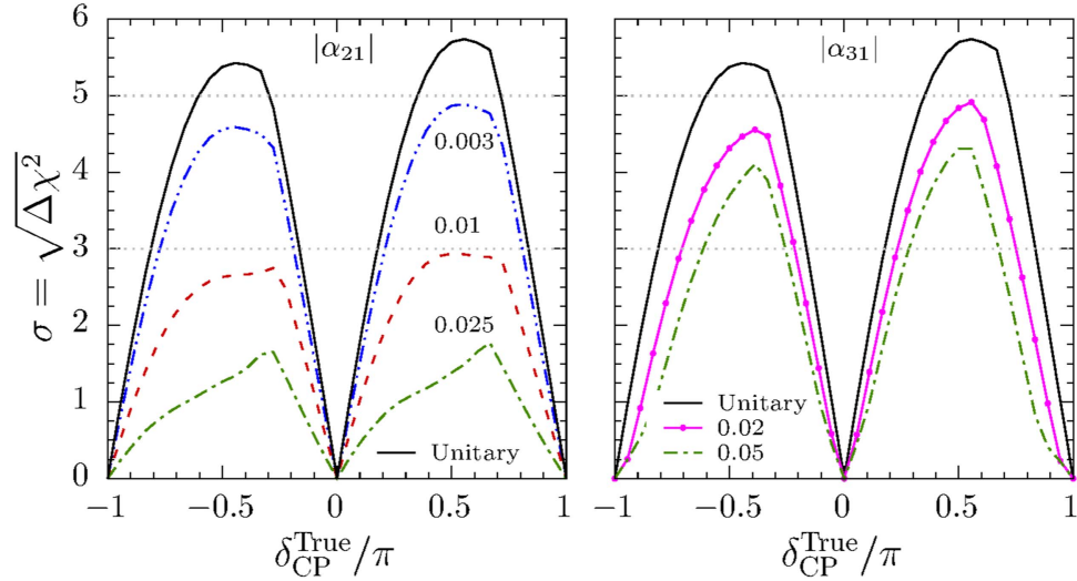
Figure 4. DUNE sensitivity to CP violation for non-unitary neutrino mixing. For comparison the black solid line shows the CP-sensitivity in DUNE, for the standard unitary case. The reduced sensitivities for non-zero \alpha_{21} ( \alpha_{31} ) are shown in the left (right) panel. All undisplayed parameters have been marginalized over, including the non-unitarity phases as well as the diagonal parameters \alpha_{ii} .
