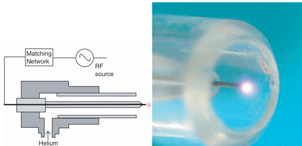
Figure 2. Schematic drawing of the plasma needle set-up (left) and plasma generated by the plasma needle (right) [53].
